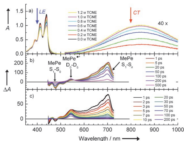
Figure 2. a) Electronic absorption spectra of 4 mM MePe and TCNE in ACN solution (thickness 100 \mu\text{m} ). The arrows indicate the spectral positions of the pump pulses for the LE and CT transitions (the latter has been multiplied by a factor of 40 for clarity). Transient UV/Vis difference absorbance spectra \Delta A measured at different pulse delays after local excitation and plotted for TCNE quencher concentrations of b) 0.1 and c) 0.9 M show the substantial spectral overlap of the excited-state absorption and stimulated emission bands, and the absorbance of the radical cation.
